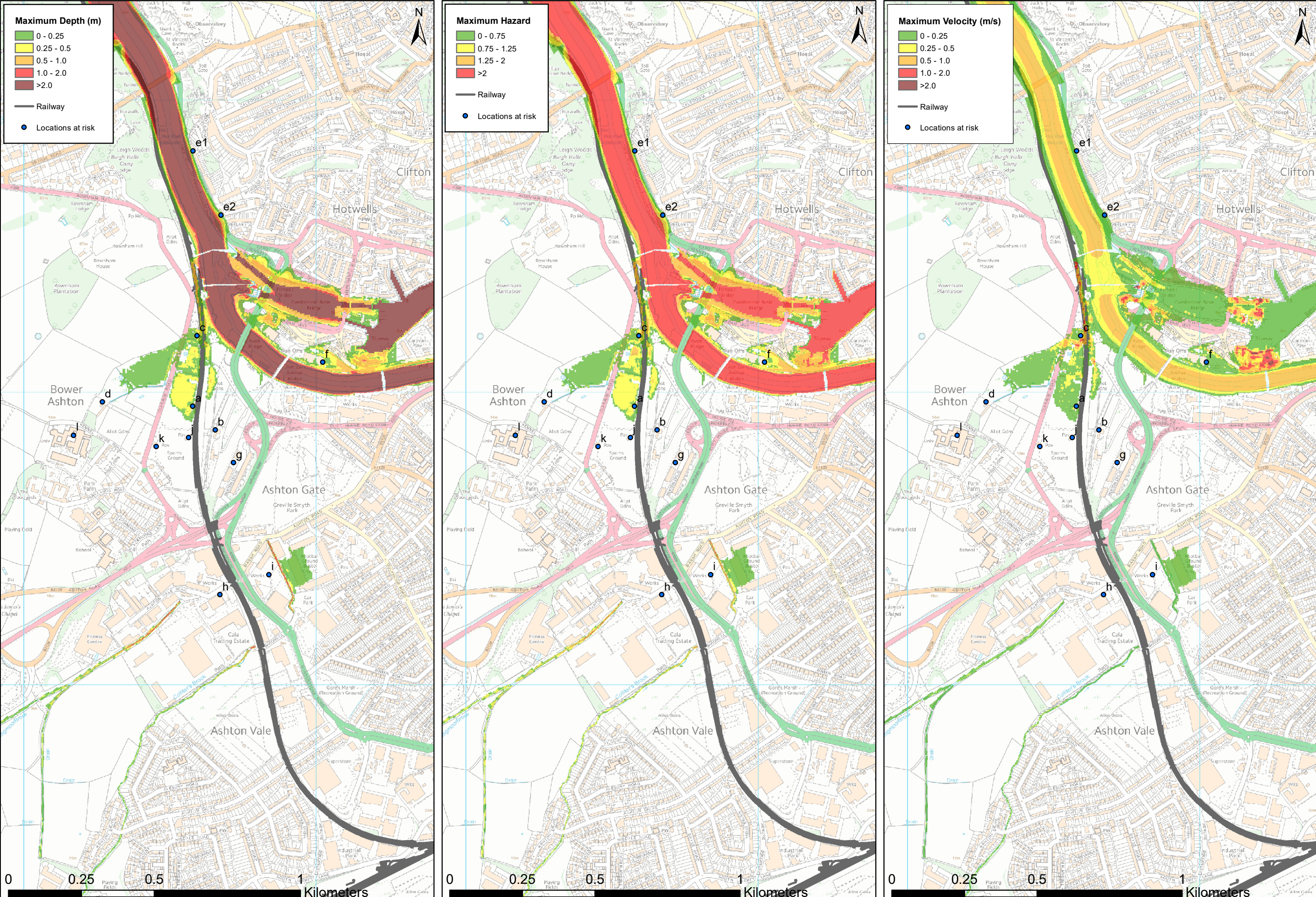
Figure N-6: Post Development, 75year rerturn period event in 2015 ,Tidal
