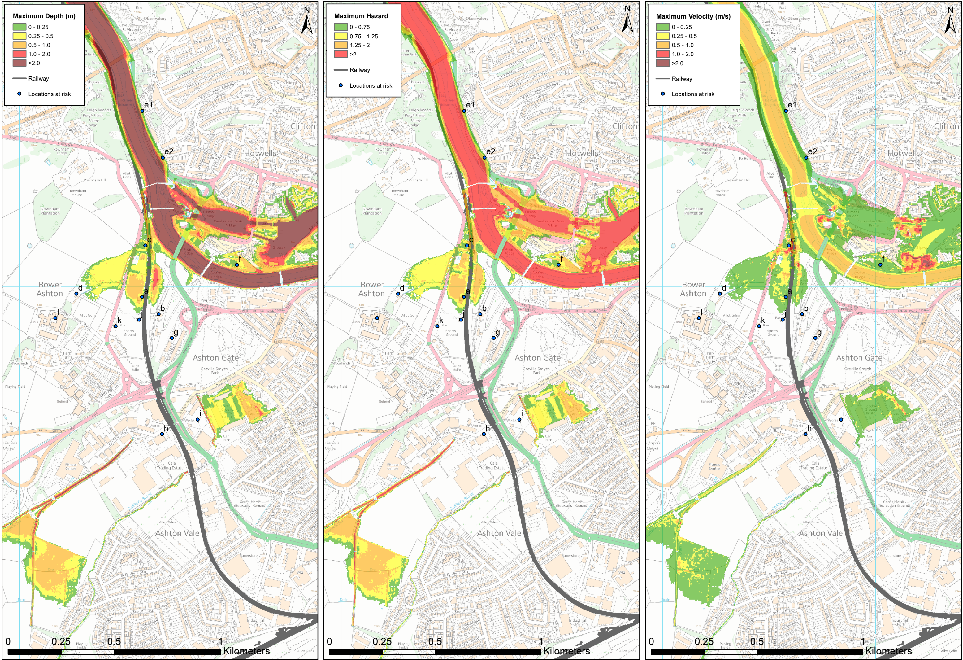
Figure N-7: Pre Development, 200year return period event in 2015 ,Tidal
