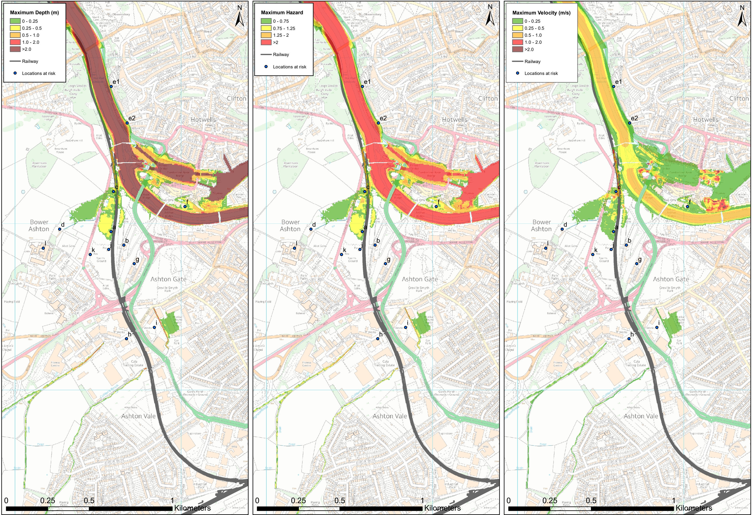
Figure N-5: Pre Development, 75year return period event in 2015 ,Tidal
