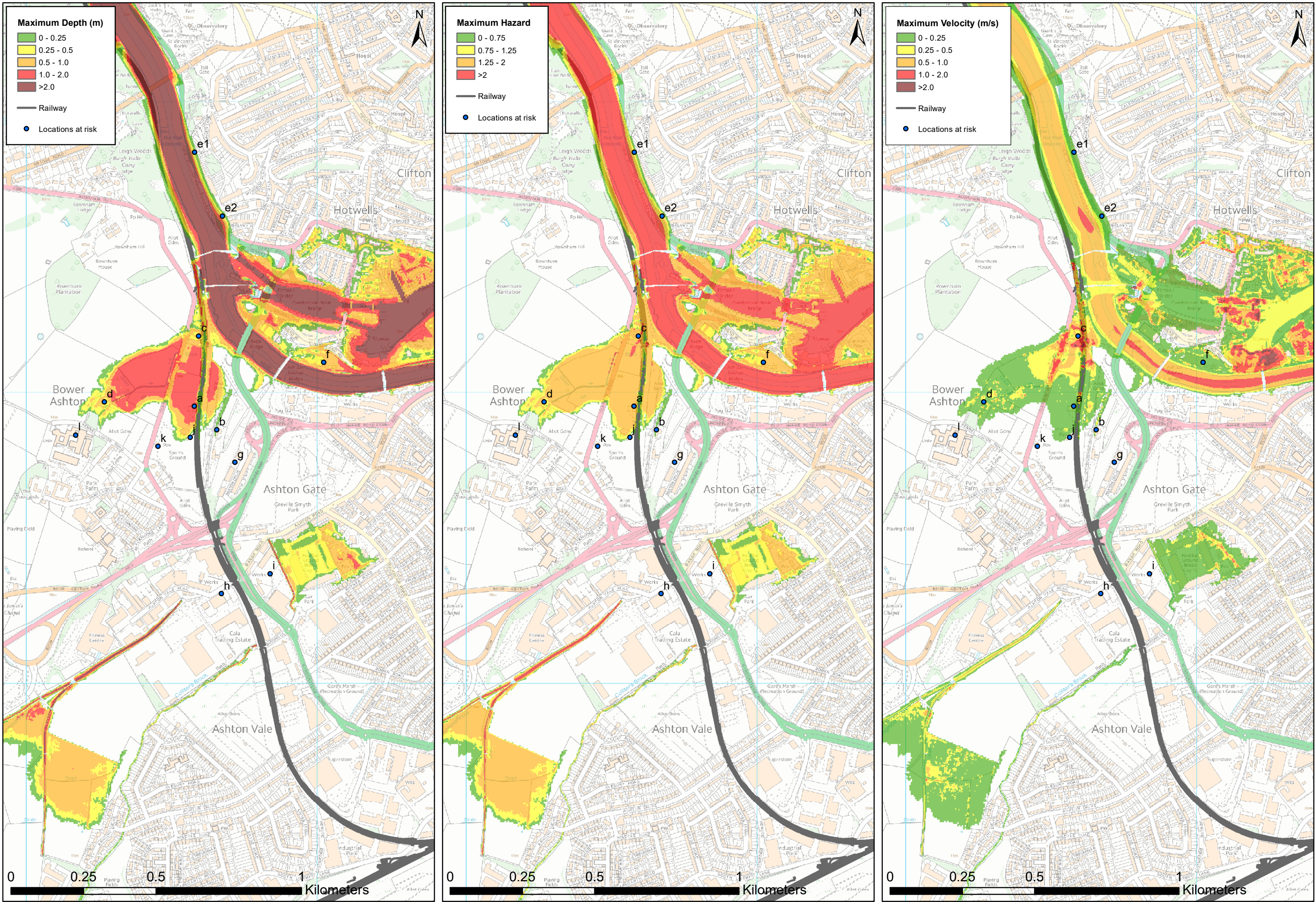
Figure N-9: Pre Development, 1000year rerturn period event in 2015 ,Tidal
