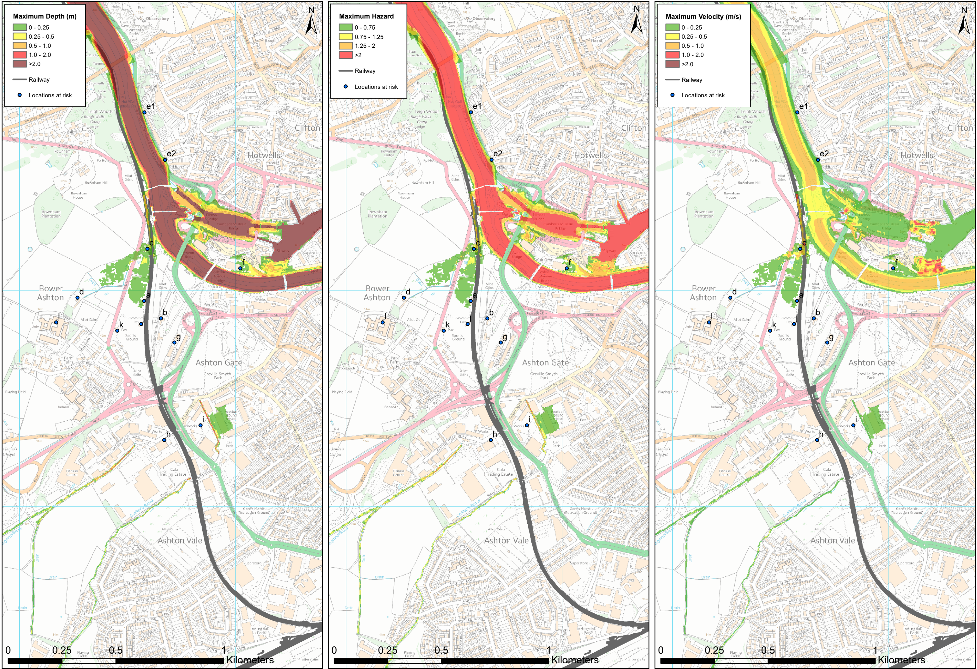
Figure N-4: Post Development, 20year rerturn period event in 2015 ,Tidal
