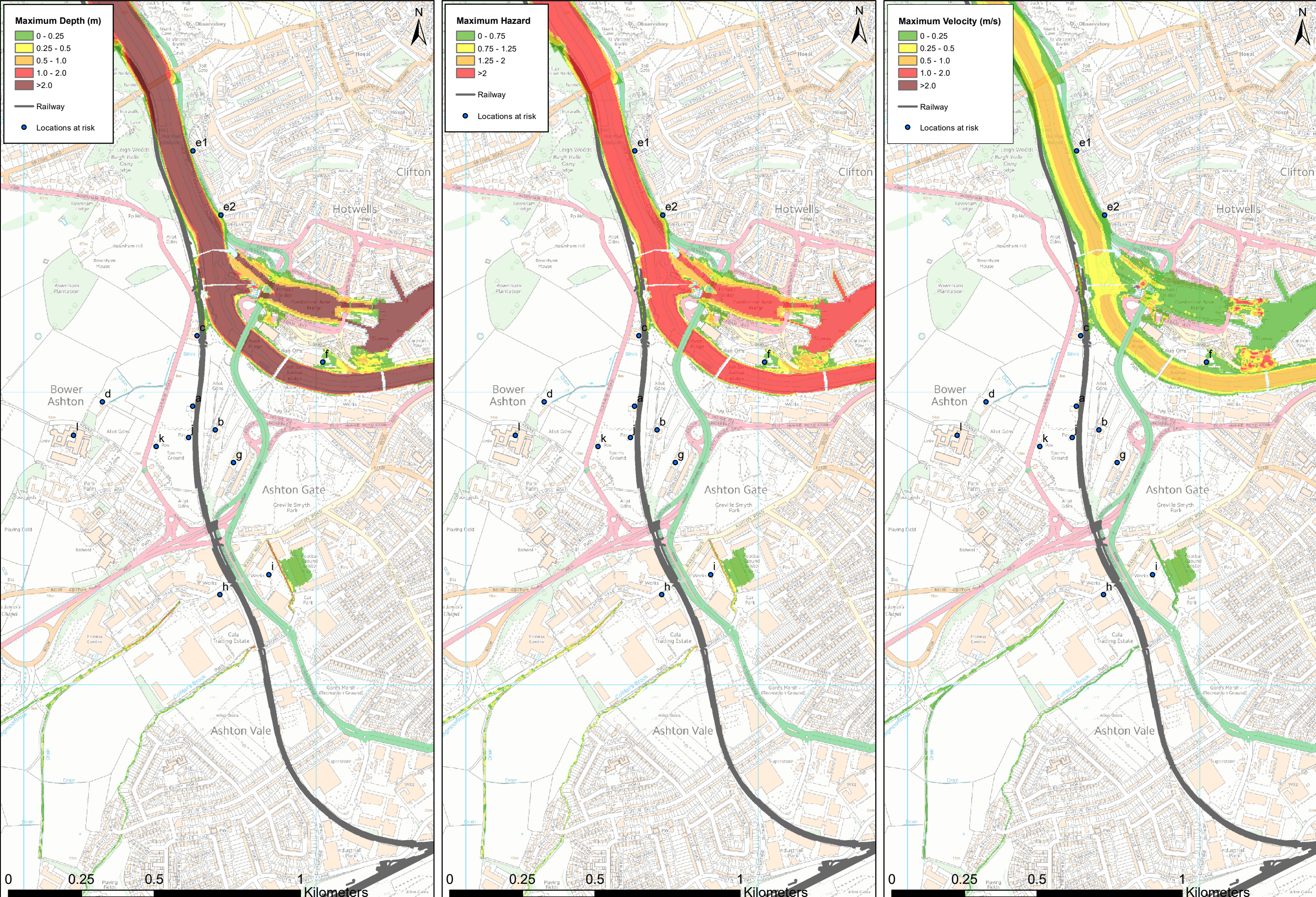
Figure N-2: Post Development, 10year rerturn period event in 2015 ,Tidal
