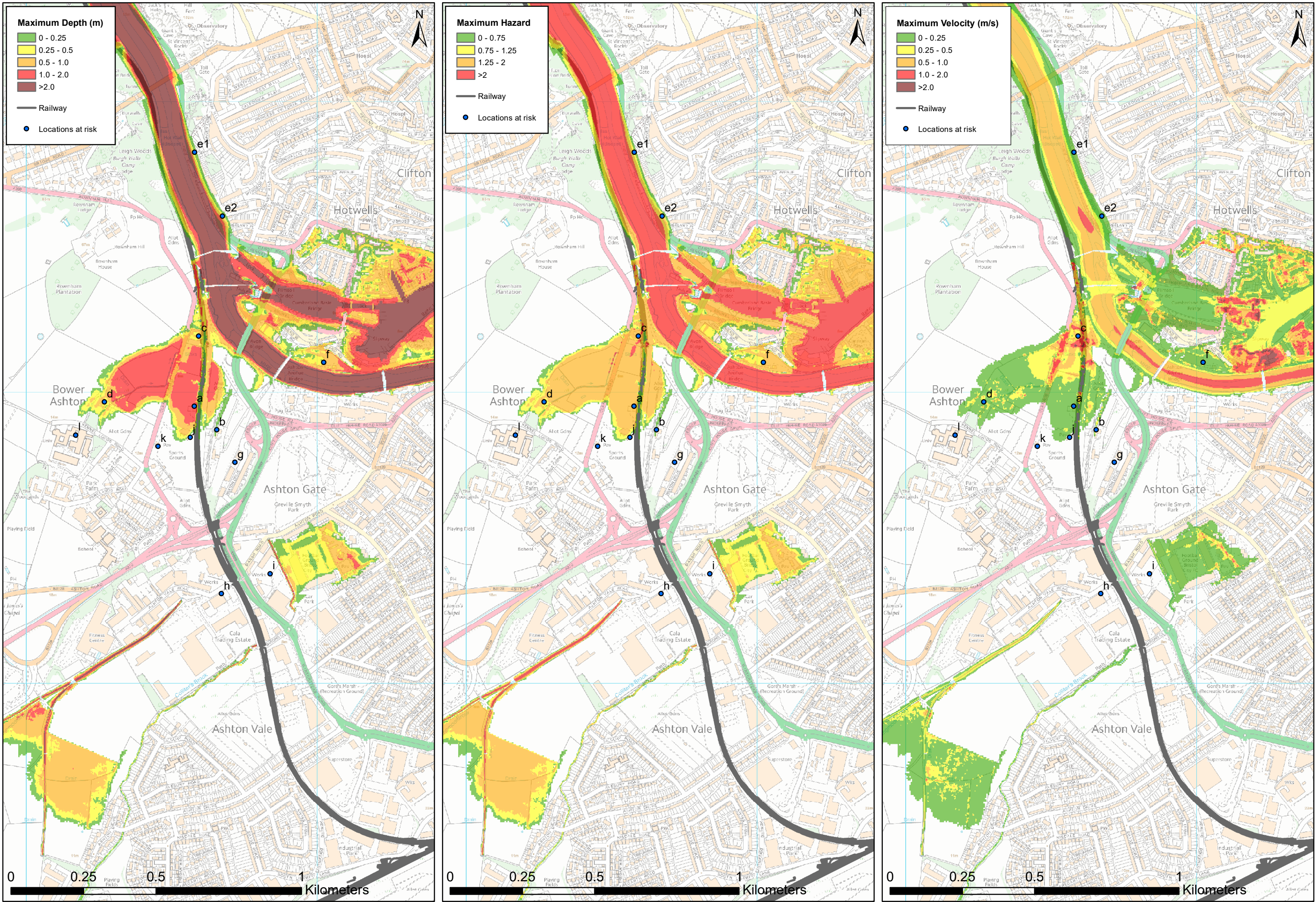
Figure N-10: Post Development, 1000year return period event in 2015 ,Tidal
