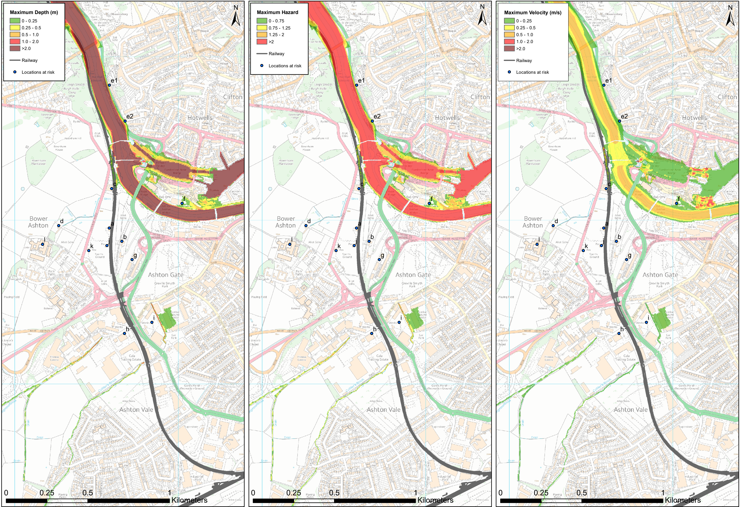
Figure N-1: Pre Development, 10year return period event in 2015 ,Tidal
