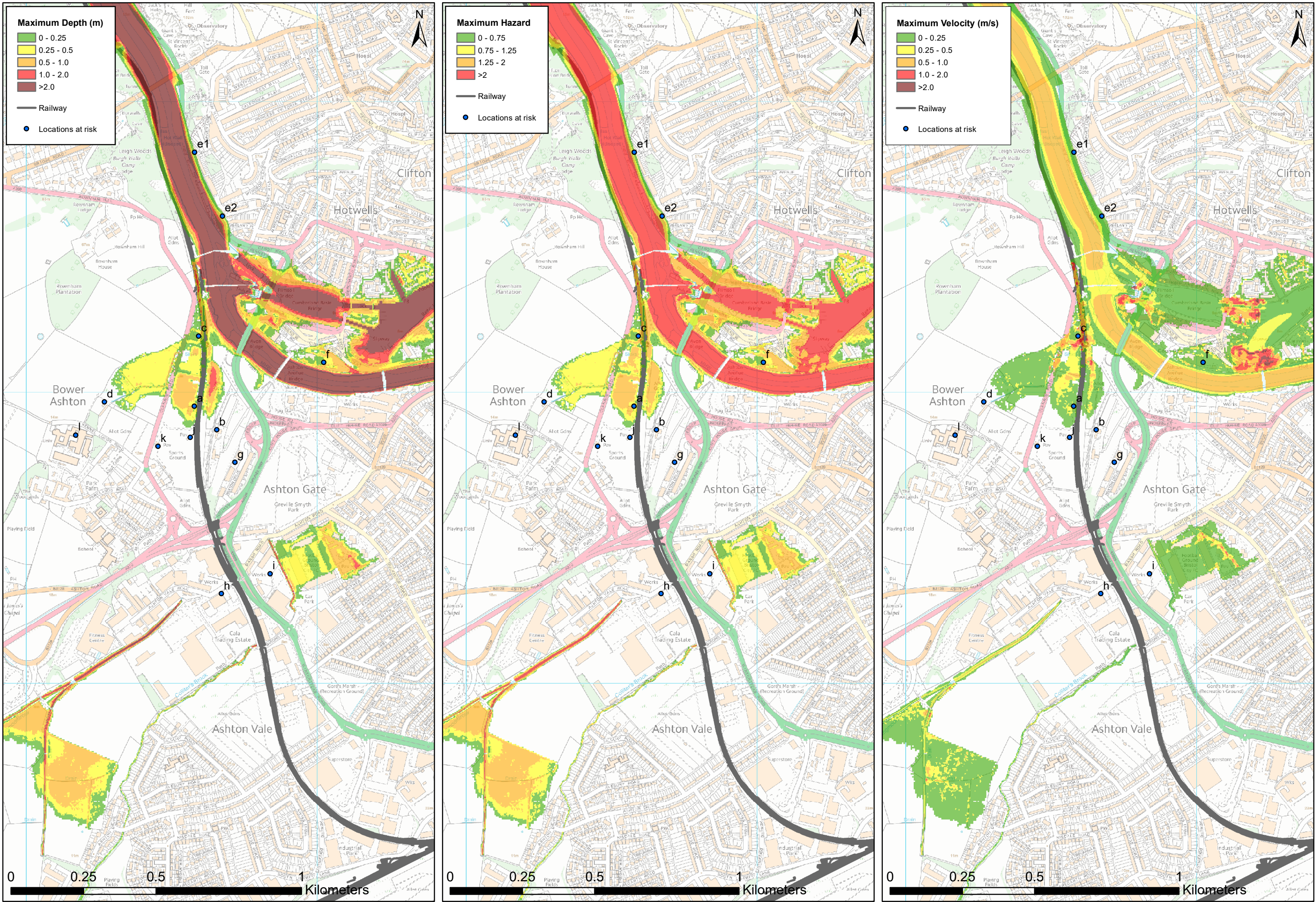
Figure N-8: Post Development, 200year rertun period event in 2015 ,Tidal
